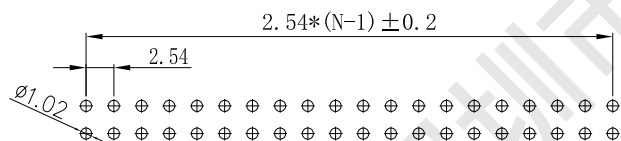
PCB LAYOUT
