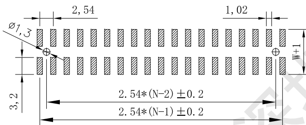
PCB LAYOUT
