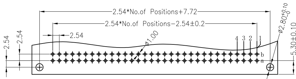
PCB LAYOUT(RECOMMENDED) (TOP VIEW TOL. :±0.05)
